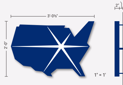
(1) 2'-0" x 3'-0 1/2" x 2" Deep Halo Illuminated Logo
